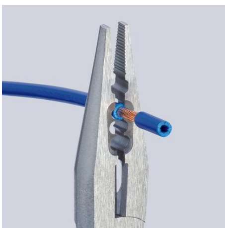
Stripping 0.5 - 0.75 / 1.5 / 2.5 mm²
