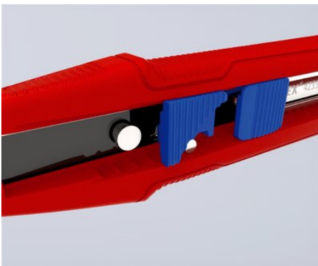
Tension-resistant blade lock and blade locking pin made from hardened steel
